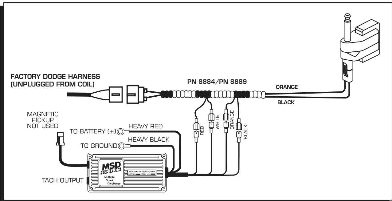
Figure 2 Installation with an MSD 6 or 7 Series Ignition Control.
