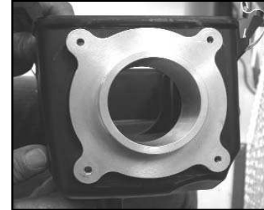
15. Install the provided adapter into the air box. Make sure the holes line up.
