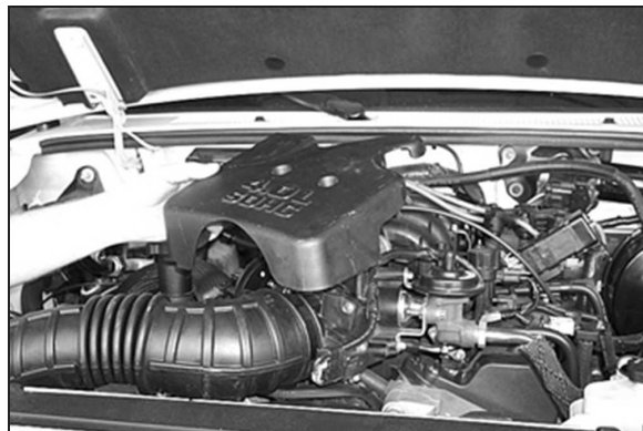
3. Loosen and remove the three bolts that secure the throttle body cover, then remove the cover as shown.
